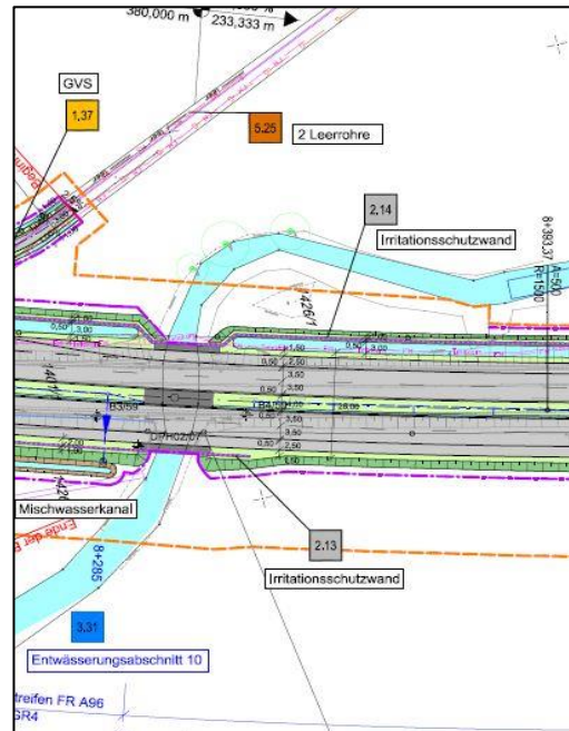
Abb. 3: BW 49-3, Bau-km 8+3000: Gennach-Brücke
